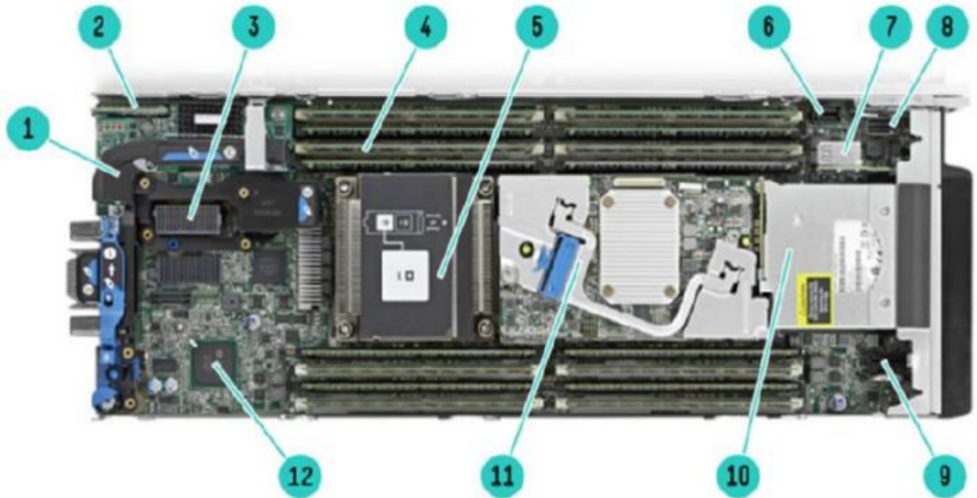
HPE ProLiant BL460c Gen9 Server Blade – Internal View
